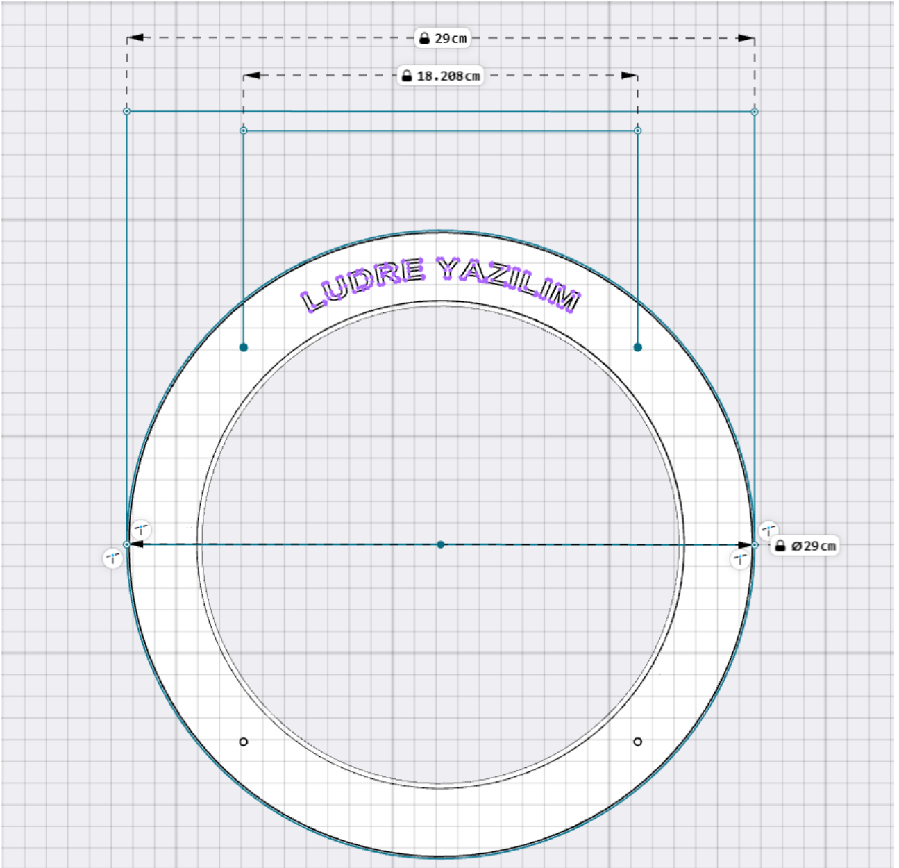
Figure 4.1. Dark Field DF22 Mounting Hole Size
