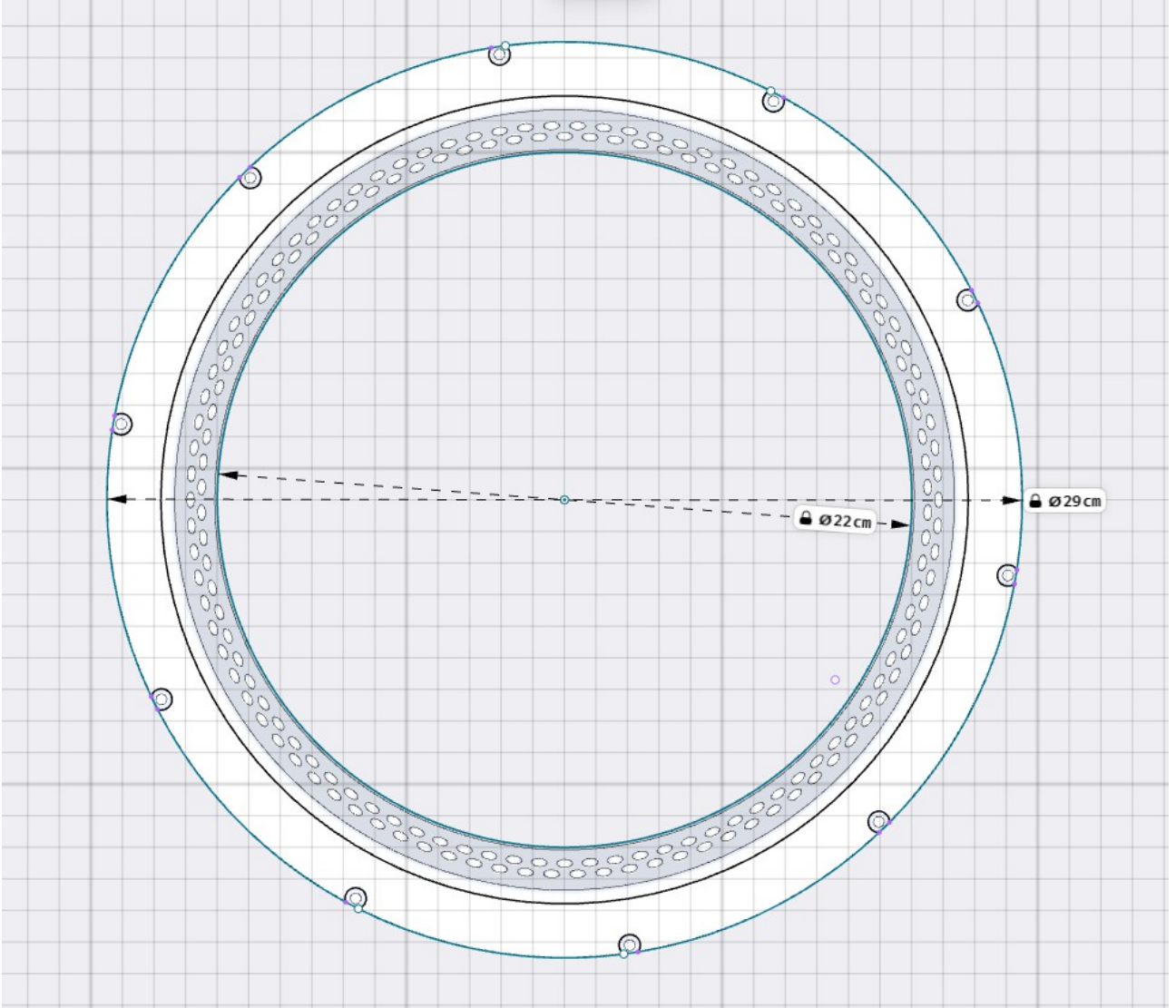
Figure 4. Dark Field DF22 Rmin&Rmax Dimensions
